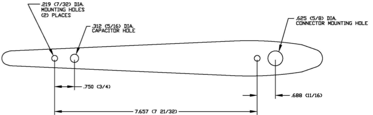
MOUNTING INFORMATION
