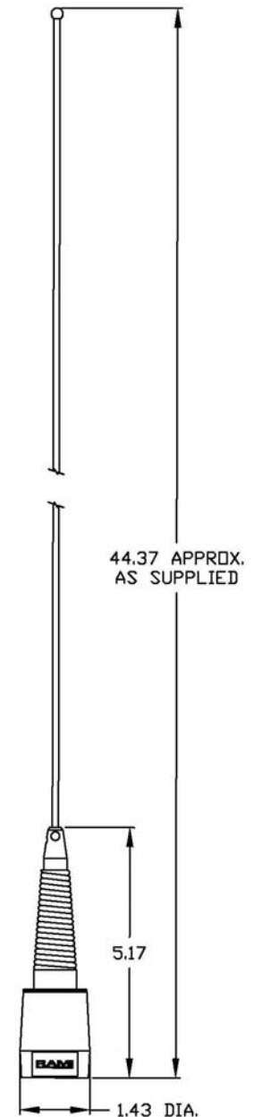
VHF WIDEBAND MOBILE ANTENNA RAMI P/N: AV-7-1A IF PURCHASED SEPARATELY
