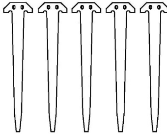
ANCHOR STAKE P/N: RAMI50-50 (4) REQ'D. + (ONE) SPARE
