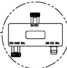
DIPLEXER SUPPLIED WITH RAMI354EX-CA
