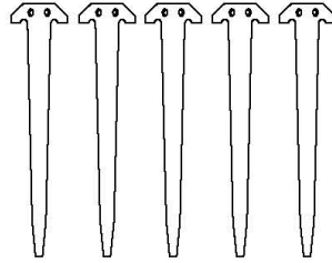
ANCHOR STAKE P/N: RAMI50-50 (4) REQ'D. + (ONE) SPARE
