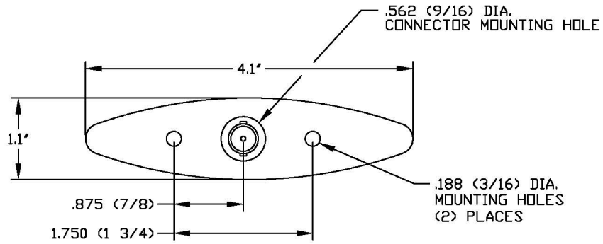
MOUNTING INFORMATION
